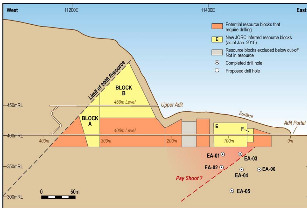
Figure 2: Pierce points of recent surface drilling at Eastern Extension
