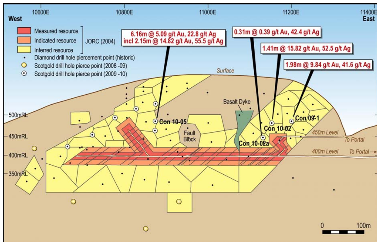
Figure 1: Results of infill drilling into Inferred Resource zone at Cononish
